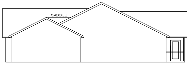
3/1 RIGHT ELEVATION SCALE: 1/8"=1'-0"
