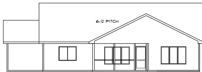
4/1 REAR ELEVATION SCALE: 1/8"=1'-0"
