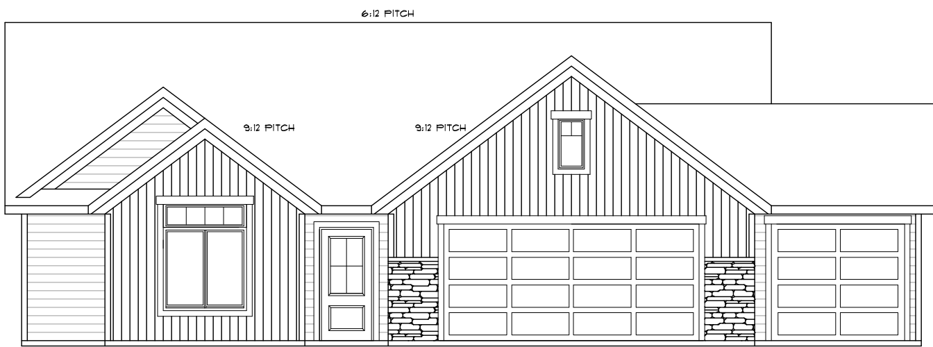
1/1 FRONT ELEVATION SCALE: 1/4"=1'-0"
